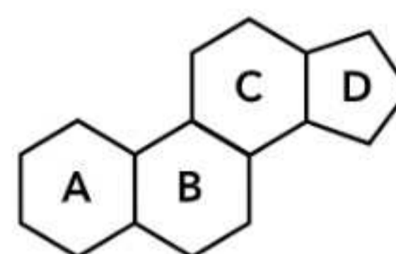
Steroid
