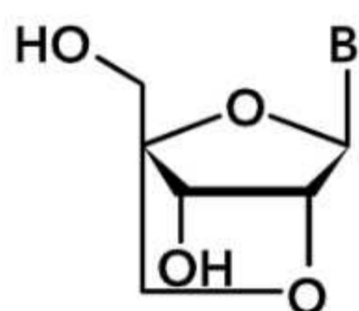
Carbohydrate
