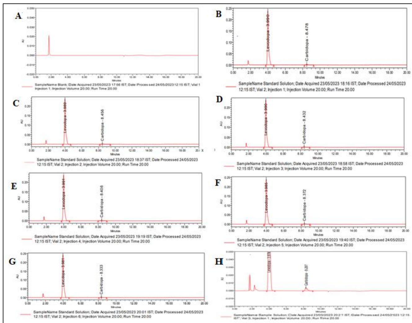
FIG. 2: ASSAY CHROMATOGRAMS: (A) BLANK; (B)STANDARD INJECTION 1; (C) STANDARD INJECTION 2; (D) STANDARD INJECTION 3; (E) STANDARD INJECTION 4; (F) STANDARD INJECTION 5; (G) STANDARD INJECTION 6; (H) SAMPLE
