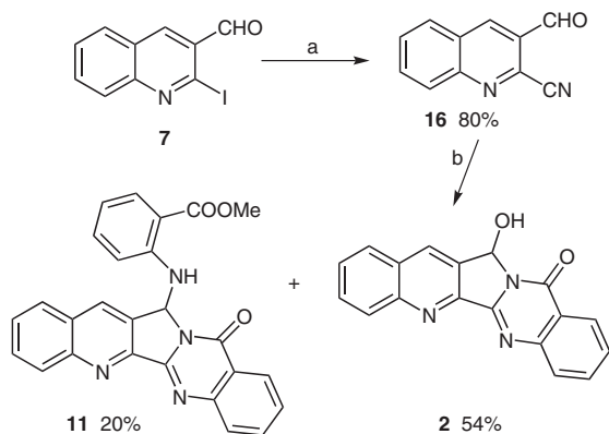
Scheme 4 Reagents and conditions: (a) CuCN, TBAB, MeCN; (b) 10 (1.05 equiv), AcOH, Ac 2 O.
