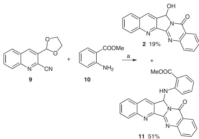
Scheme 3 Reagents and conditions: (a) AcOH, 110 °C, 12 h.
