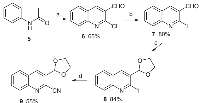
Scheme 2 Reagents and conditions: (a) DMF, POCl 3 , 70–80 °C; (b) NaI, HCl (cat.), MeCN, 80–90 °C; (c) ethylene glycol, PTSA; (d) CuCN, TBAB, MeCN, 80–90 °C.
