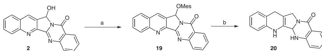
Scheme 6 Reagents and conditions: MesCl, Et 3 N, CH 2 Cl 2 ; (b) Pd/C (10%), MeOH.
