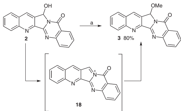
Scheme 5 Reagents and conditions: MeOH, Amberlyst or MeOH, Indion resin, 60 °C.
